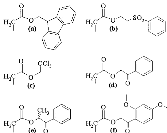
Scheme 2. Protecting groups tested for Glu or Asp side chain protection: OFm (a), OPse (b), OTce (c), OPac (d), OMop (e), and OdiMeOPac (f)
