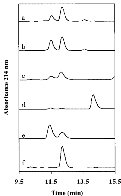
Figure 2. HPLC analysis of ligation products using different H-LYRAD(X)-sr peptides: (a) ligation between substrates 1 and 3 ; (b) ligation between substrates 1 and 3 co-injected with compound 6 ; (c) ligation product between substrates 15 and 3 after basic treatment; (d) ligation product between substrates 14 and 3 ; (e) ligation product between substrates 14 and 3 after basic treatment; (f) ligation product between substrates 16 and 3 after \text{Zn}^0 reduction
