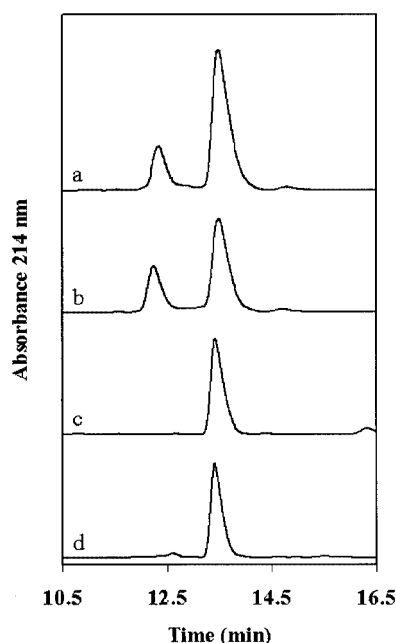
Figure 1. HPLC analysis of ligation products using different H-LYRAE(X)-sr peptides: (a) ligation between 2 and 3; (b) ligation between substrates 2 and 3 co-injected with compound 7; (c) ligation product between substrates 8 and 3 after basic treatment; (d) ligation product between substrates 9 and 3 after basic treatment
