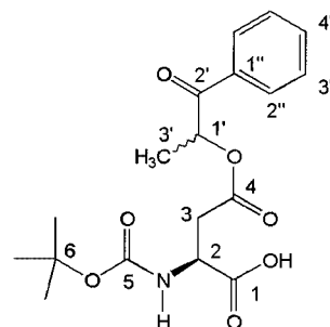
Figure 3. Structure of Boc-Asp(OMop)-OH
